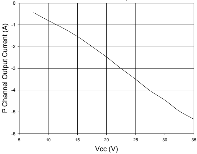
Vcc vs. P Channel Output Current
