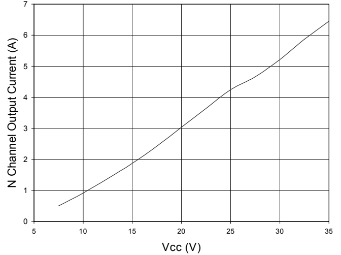
Vcc vs. N Channel Output Current
